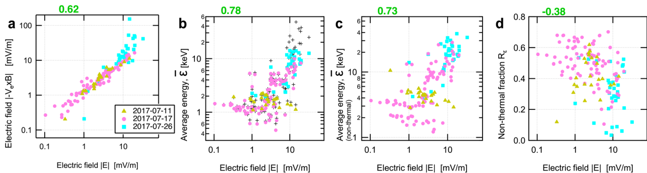
FIG. 8. Comparison between electric field magnitude |E| and four different parameters: (a) the electric field calculated from |\mathbf{-V}_e \times \mathbf{B}| , (b) average energy of electrons \bar{\epsilon} , (c) the same as (b) but for non-thermal electrons, and (d) non-thermal fraction of electron energy R_e . The data points are obtained by averaging the data over 30 s and by applying spectral fitting for each averaged data. The black plus signs in panel (b) are obtained from the FPI electron moment data. Correlation coefficients are annotated on the upper left corners.
