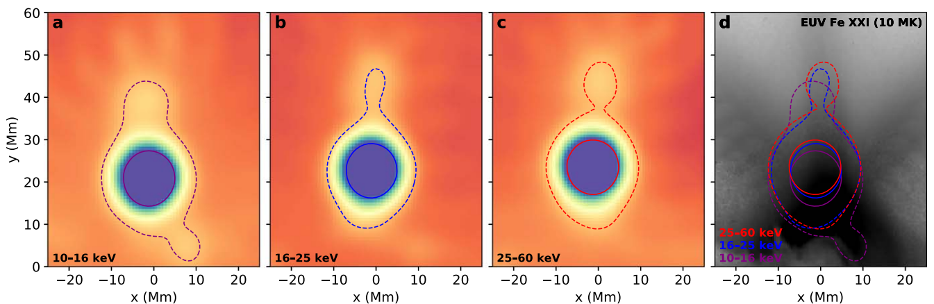
Figure 11. RHESSI X-ray images for the time of interest on 2017 September 10. The time interval used for imaging is 16:10:00–16:11:10 UT. The energy ranges used for imaging are 10–16 keV, 16–25 keV, and 25–60 keV, shown in panels (a), (b), and (c), respectively. The solid and dashed lines denote the 50% and 10% contours. Panel (d) shows X-ray images of all three energy ranges overlaid on the SDO/AIA 131 Å (Fe XXI) EUV image at the closest time (shown in reversed gray scale).
