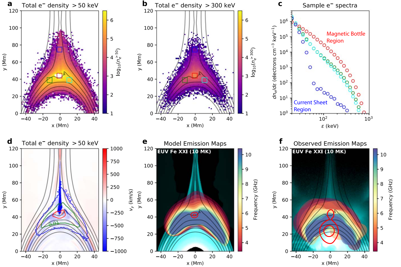
Figure 8. Distribution of nonthermal electrons around the magnetic bottle region and the associated emissions. (a) and (b) are spatial distribution of > 50 keV and > 300 keV electrons, respectively. Note that they are shown on a logarithmic scale. (c) Example model nonthermal electron spectra from four regions marked in panels (a) and (b), with one located near the Y point (red), two in the loop legs (green and cyan), and one in the current sheet region (blue). (d) Contours of > 50 keV electron distribution overlaid on the model v_y map. Blue, green, and red contours are 0.1%, 1%, and 15% of the peak electron density, respectively. In particular, the innermost red contour encloses 51% of all the > 50 keV electrons. (e) Synthetic SDO/AIA (background), 25–60 keV HXR (red contours), and multifrequency microwave sources (filled color contours) as calculated from the combined MHD and particle model. (f) Multifrequency observations identical to Figure 3(d), overlaid with magnetic field lines derived from the model.
